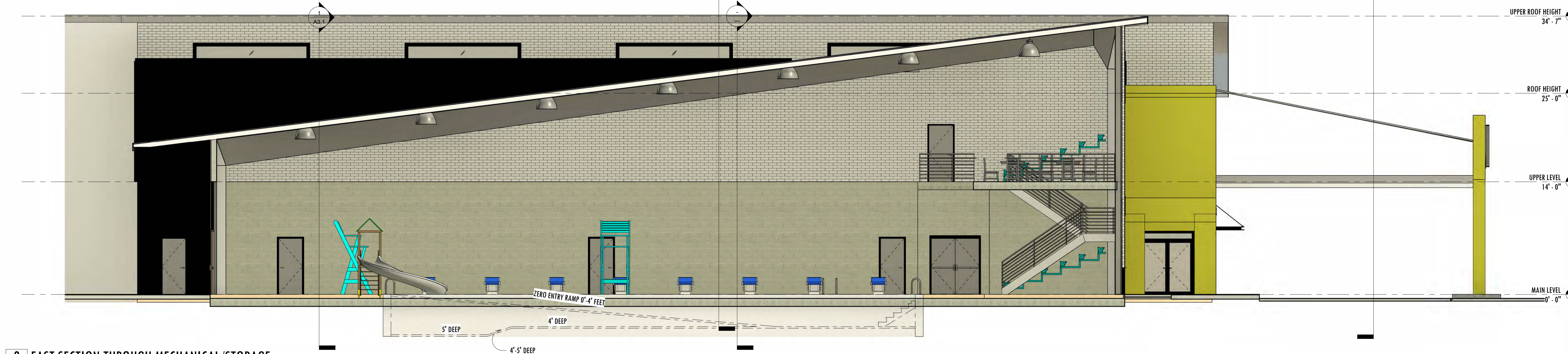
3 EAST SECTION THROUGH MECHANICAL/STORAGE A3.1 3/16" = 1'-0"
